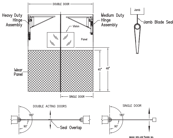
Standard 2600 Vinyl Door
