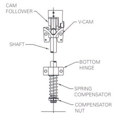
Hinge Detail
